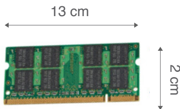
Laptop RAM
